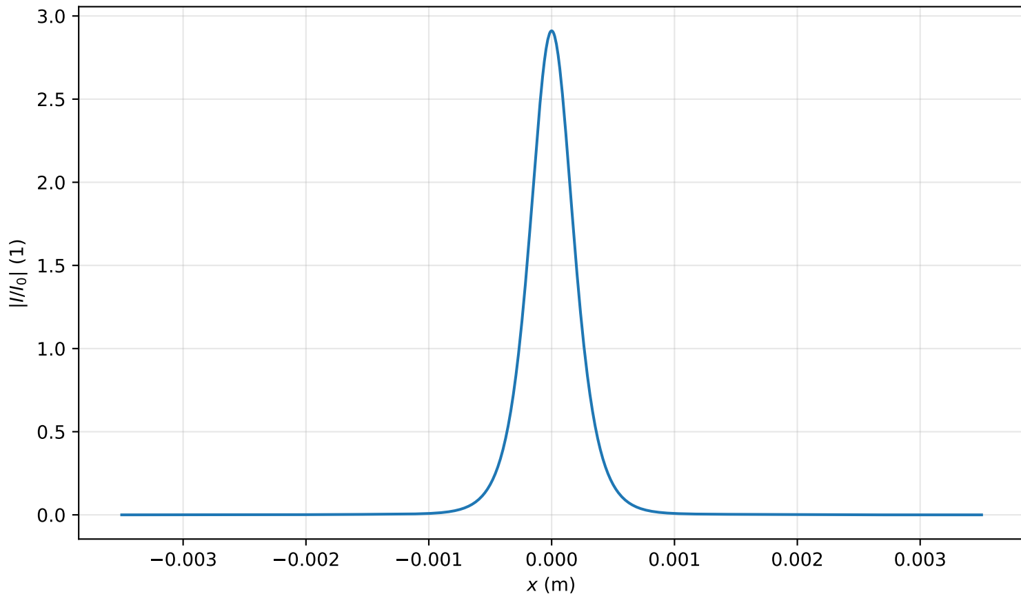
Intensity profile I(x, y = 0, z = 3.423m)/I_0 , P_{in}=1.0P_{cr} , artificial time
